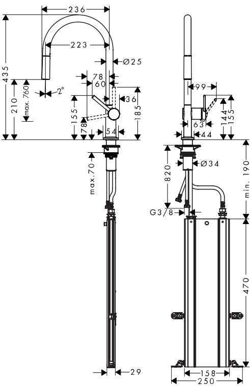
Talis M54 210 1jet sBox 72848000
